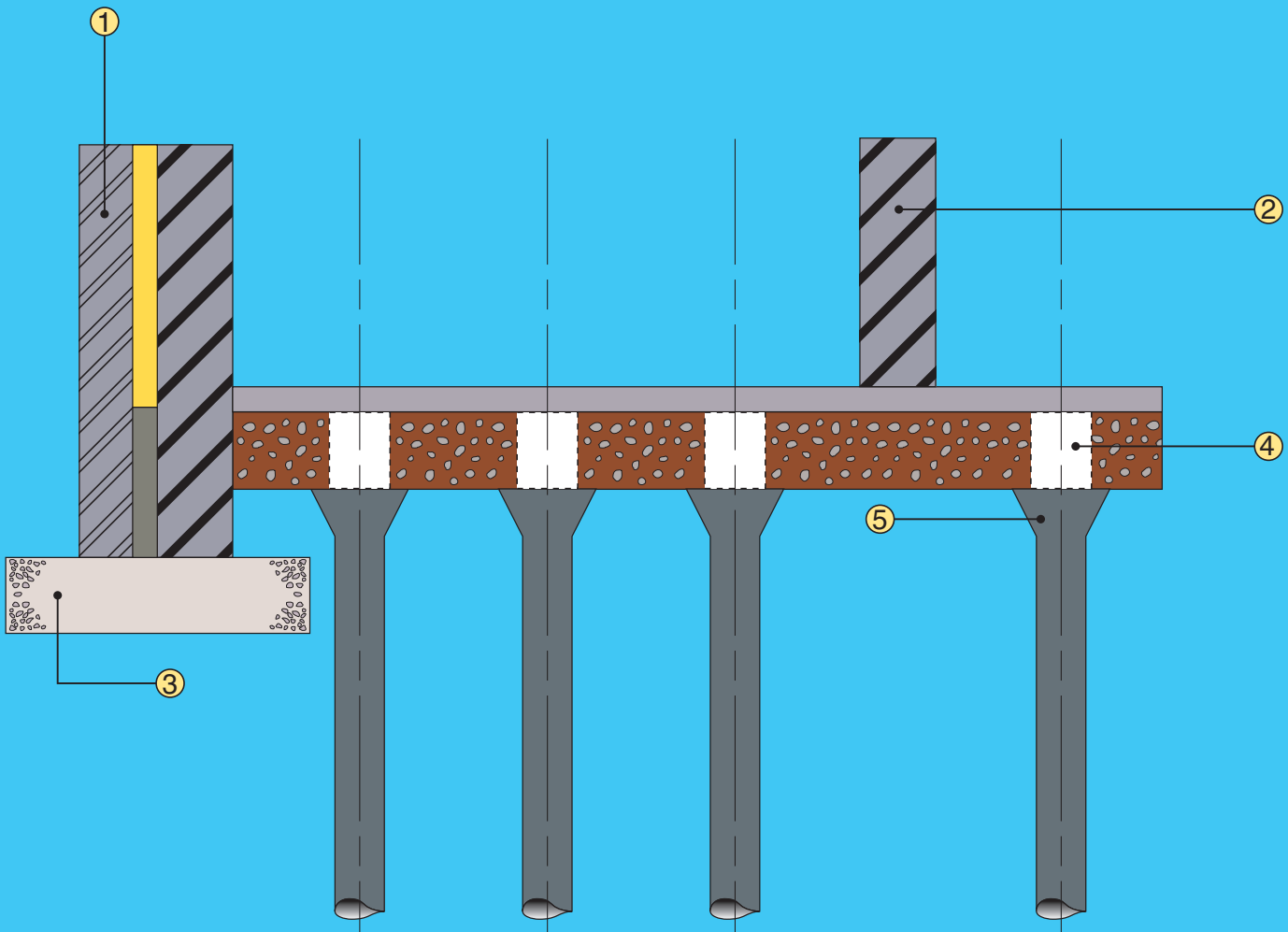
Typical Section
