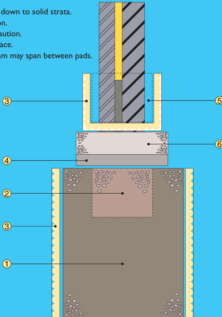
Typical Section
